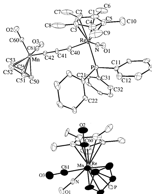
Figure 3. Structure of the cation of 9 -(CH 2 Cl) 0.5 (top) and Newman-type projection down the manganese–rhenium linkage (bottom).
