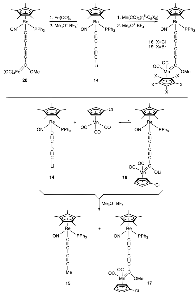
Scheme 4. Syntheses of C 5 Ome Complexes
